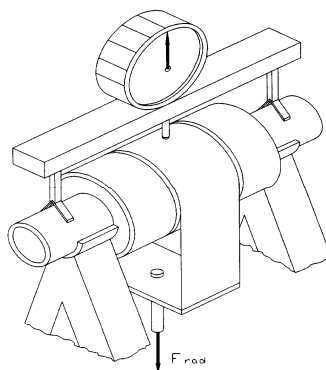
Figure 5 — Measuring arrangement for radial displacement
